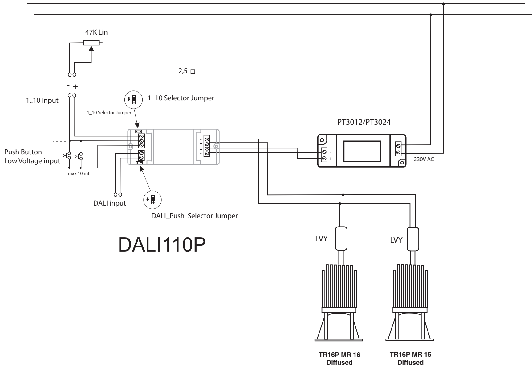
1..10V & Push button DALI system driving constant current TRIOPower 700mA
